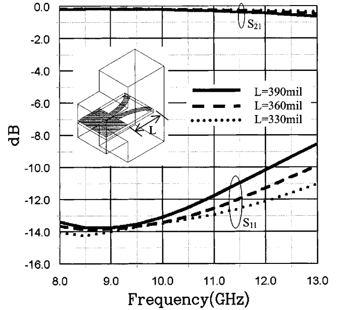
Fig. 2. Simulated results for slotline-to-waveguide transition with length of tapered slotline probe as a parameter.
