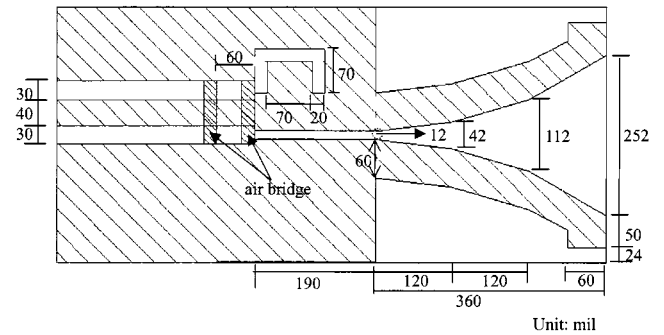
Fig. 3. Layout and dimensions of the planar circuit in the transition.
